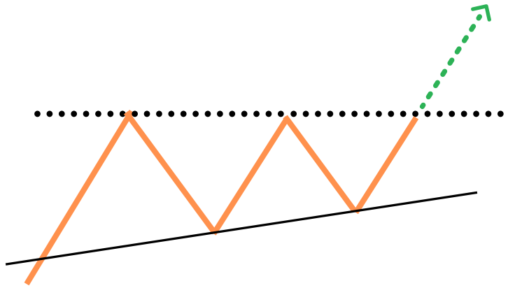
Ascending Triangle
