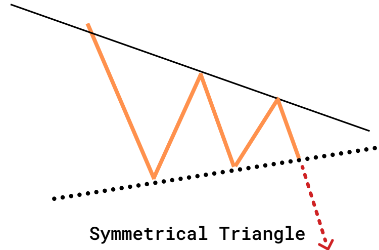
Symmetrical Triangle
