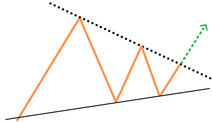
Symmetrical Triangle
